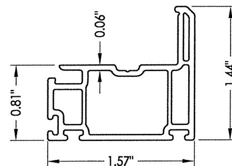
4 BOTTOM RAIL
