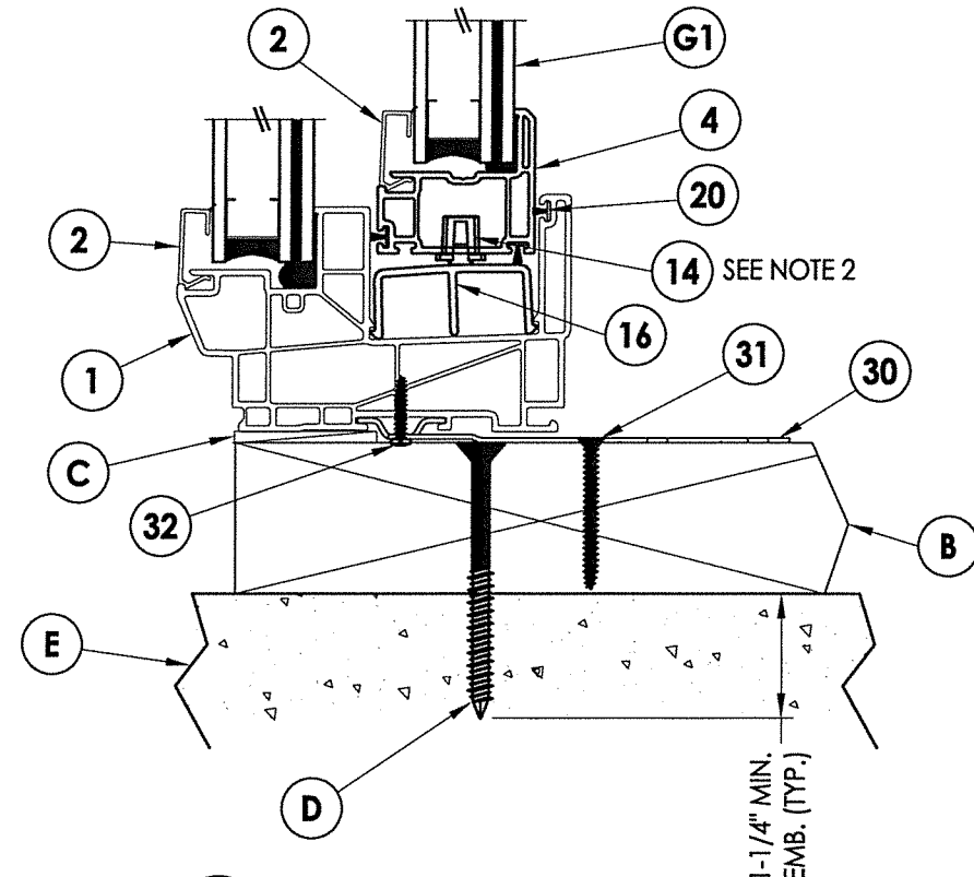
3 VERTICAL CROSS SECTION 2 2X Buck Masonry Construction
