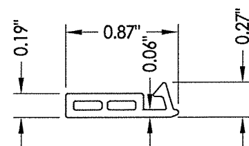
19 FLORIDA FLANGE (Optional)
