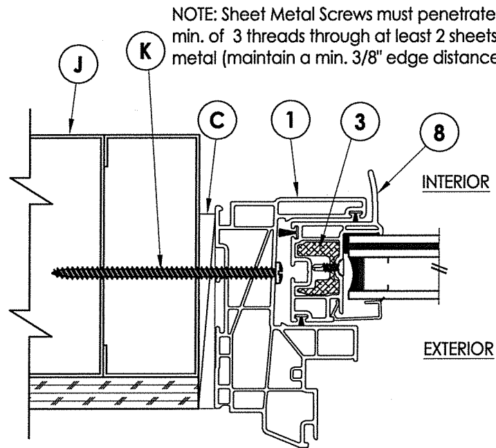
4 HORIZONTAL CROSS SECTION 2 Metal Stud Construction
